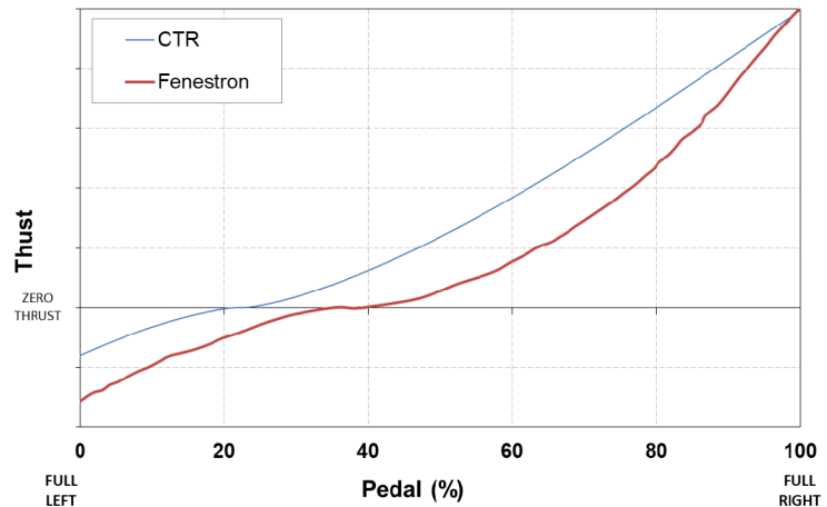
Figure 1: Comparison of Fenestron and CTR in hover
